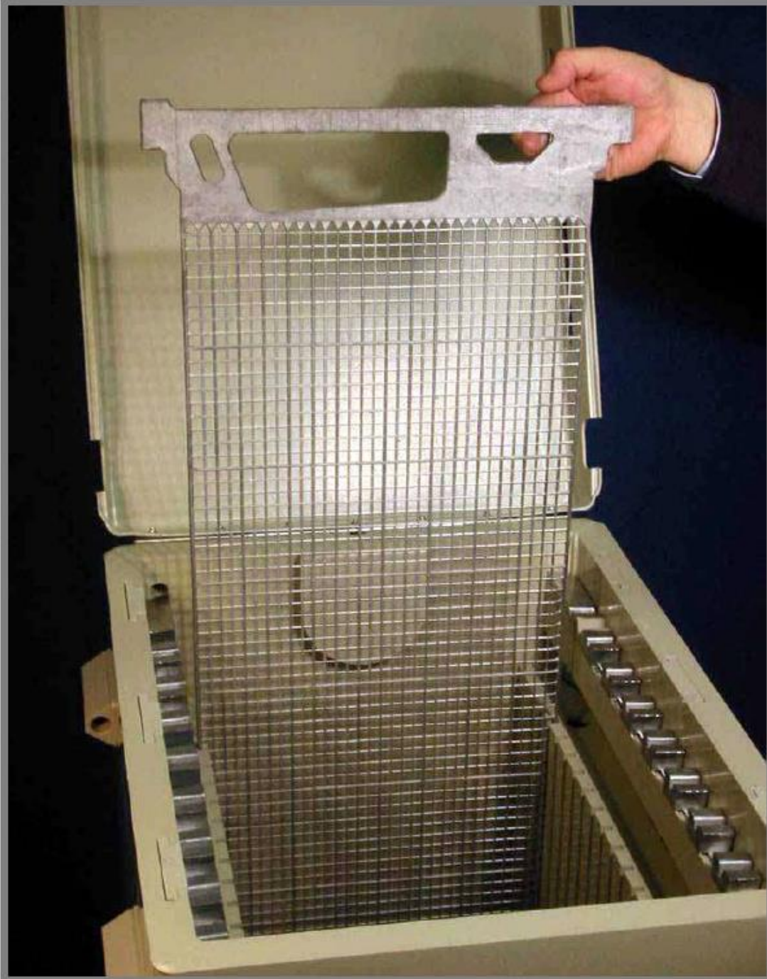
Deep Charge Plate Inserted into Formation Box
